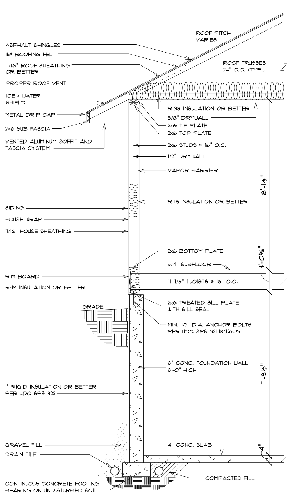
TYPICAL RANCH SECTION SCALE: 3/8" = 1'-0"
