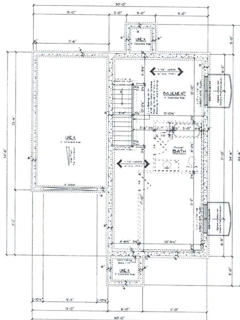
FOUNDATION PLAN 8'-0" CONCRETE WALL HGT.
