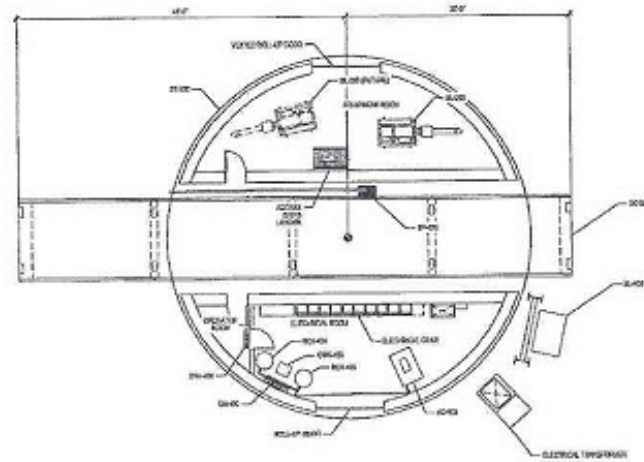
1 SILO FLOOR AT GRADE LEVEL ELEVATION
