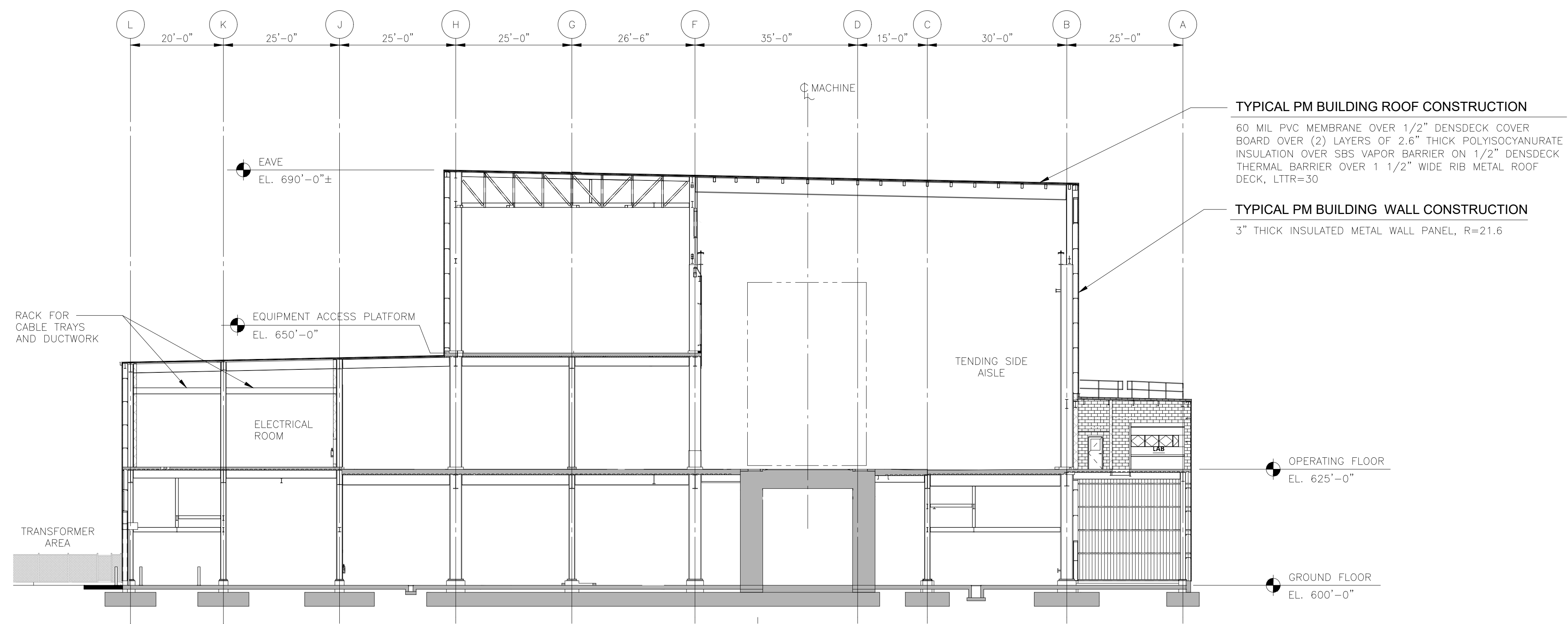
PAPER MACHINE BUILDING CROSS SECTION - VIEW LOOKING WEST
